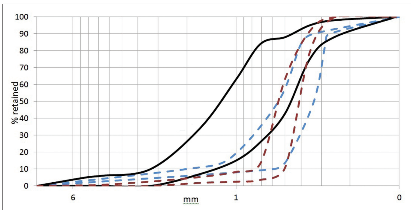
Figure 5. Particle size analysis for sediments from the North Welsh Coast. Black lines represent a grading envelope of material specified for beach recharge schemes in the area (Coastal Engineering UK Ltd, 2012), dashed red lines indicate sediment composition of sandbanks (CMACS, 2005) and dashed blue lines represent sediment composition of the sandy foreshore.
