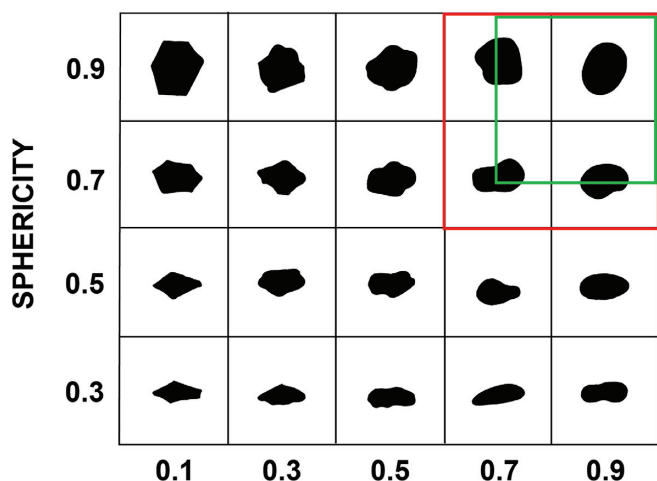
Figure 3. Chart for visual estimation of roundness and sphericity of sand grains (After Krumbein & Sloss, 1963). The red box shows the limits for frac sand and the green box for synthetic proppants.
