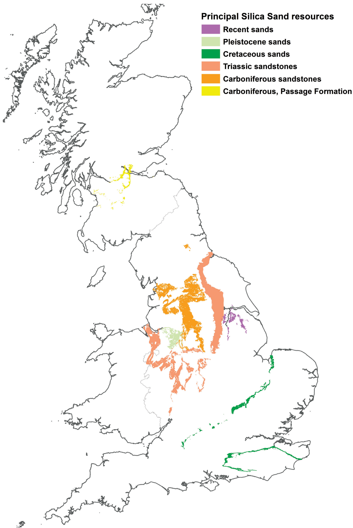
Figure 4. Principal silica sand resources in the UK. Derived map image, BGS © NERC. Contains Ordnance Survey data © Crown Copyright and database rights 2014.
